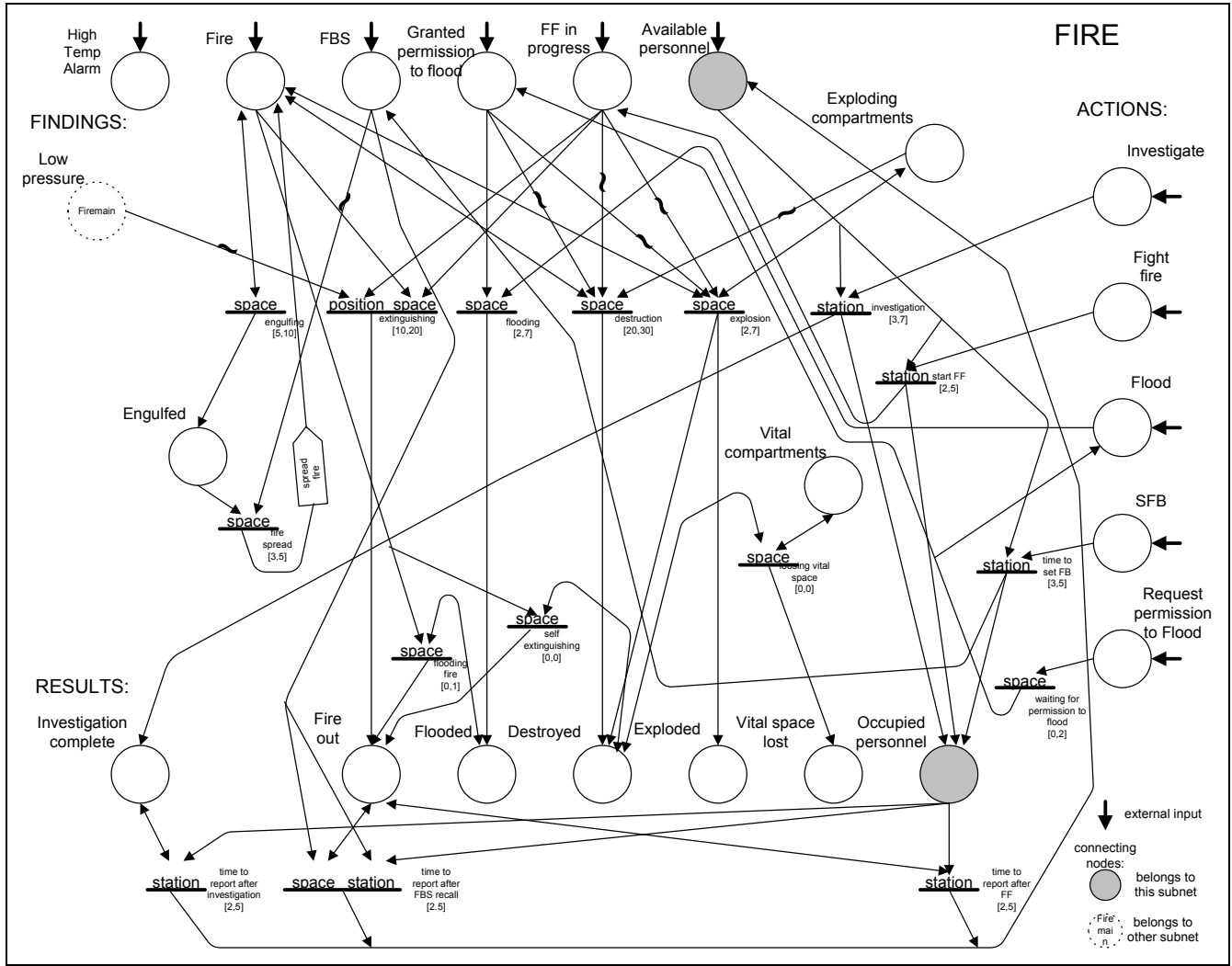
Figure 6: Time Interval Petri Network used to model fire spread in Minerva 5.2 and the experiments described in this paper.
